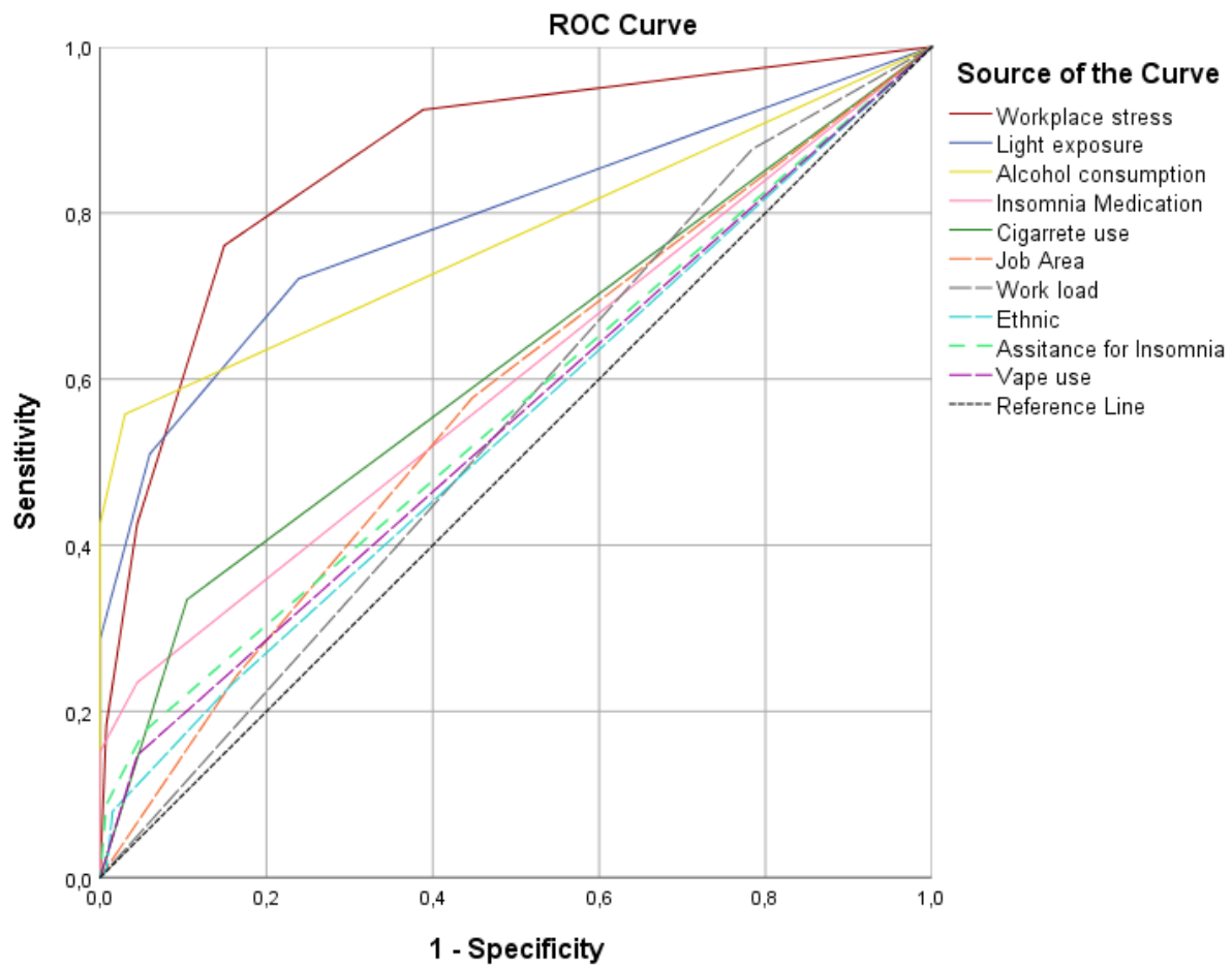
1 Figure 3: ROC Curve for Variables in Predicting Clinically Significant Insomnia
