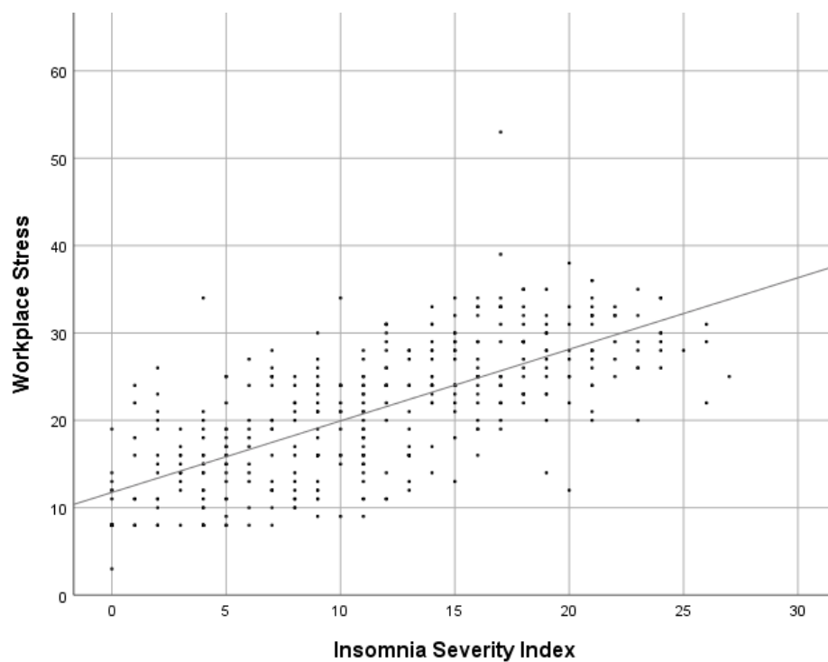
1 Figure 1. Scatter plot between Insomnia Severity Index (ISI) scores and Workplace Stress Scale (WSS) scores.
